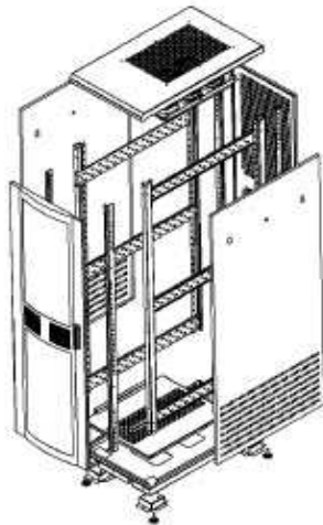
Explode View
